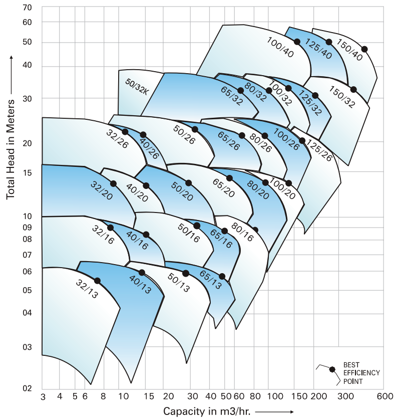
Family Curves of DB Pump at 1450 rpm-50Hz
