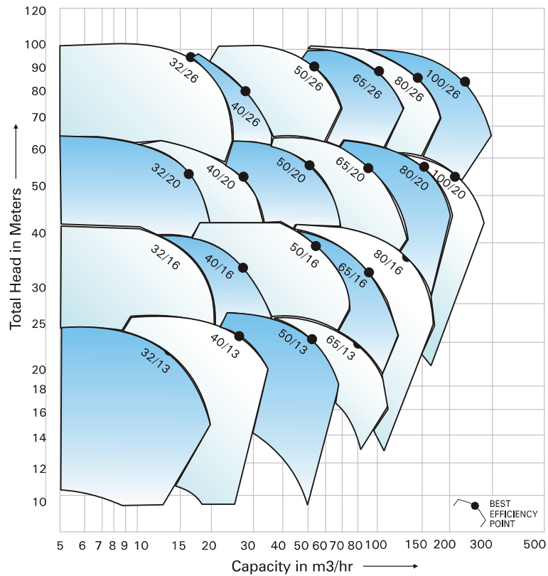
Family Curves of DB Pump at 2900 rpm-50Hz
